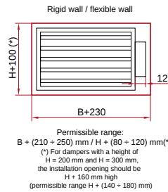
Figure 3. Openings required for the WKP-O damper
