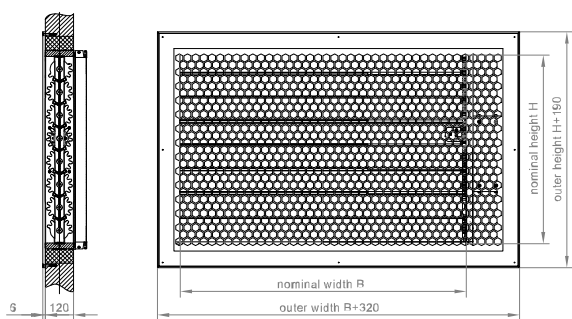
Figure 5. Flat honeycomb mesh cover
