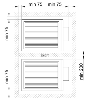
Figure 4. Spacing required between the dampers
