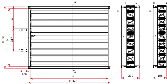
Figure 1. Dimensions of the WKP-O damper: a) WKP-O-K, b) WKP-O-KR (with a spigot on the R-side).
