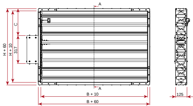
Figure 2. Dimensions of the WKP-O-T damper
