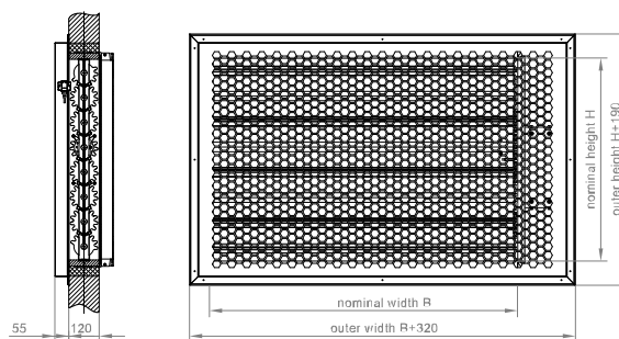
Figure 6. Convex honeycomb mesh cover
