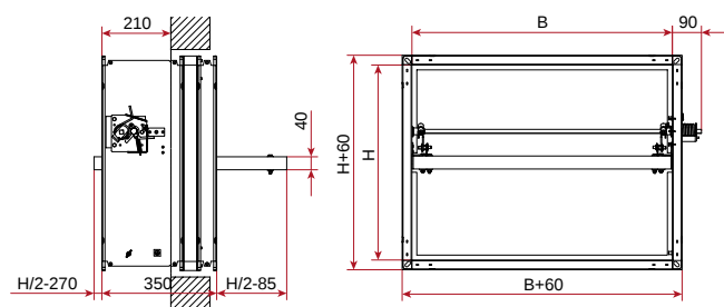
Figure 2. KWP-O-S-Ex damper (with a spring mechanism).
