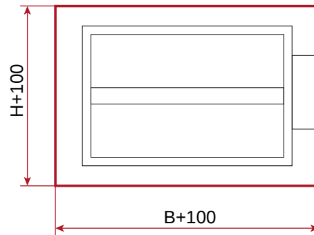
Figure 3. Openings required for the KWP-O-Ex damper.
